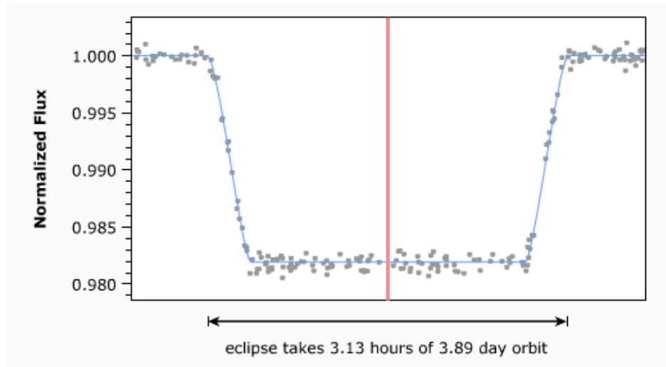
Figure 11.14: Transiting exoplanet #3.
