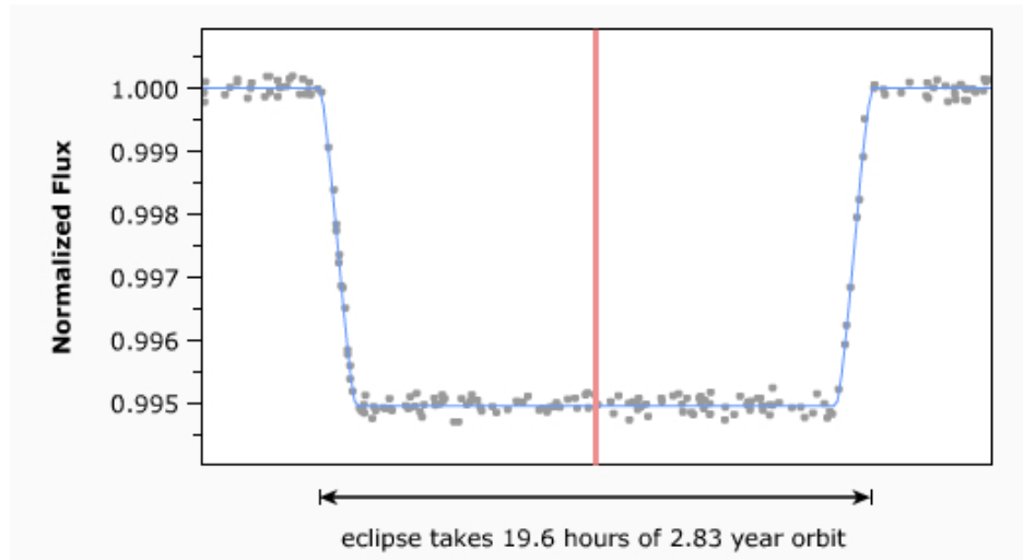
Figure 11.17: Transiting exoplanet #6.
