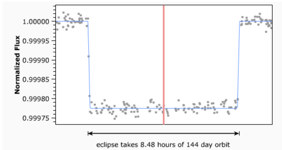
Figure 11.16: Transiting exoplanet #5.
