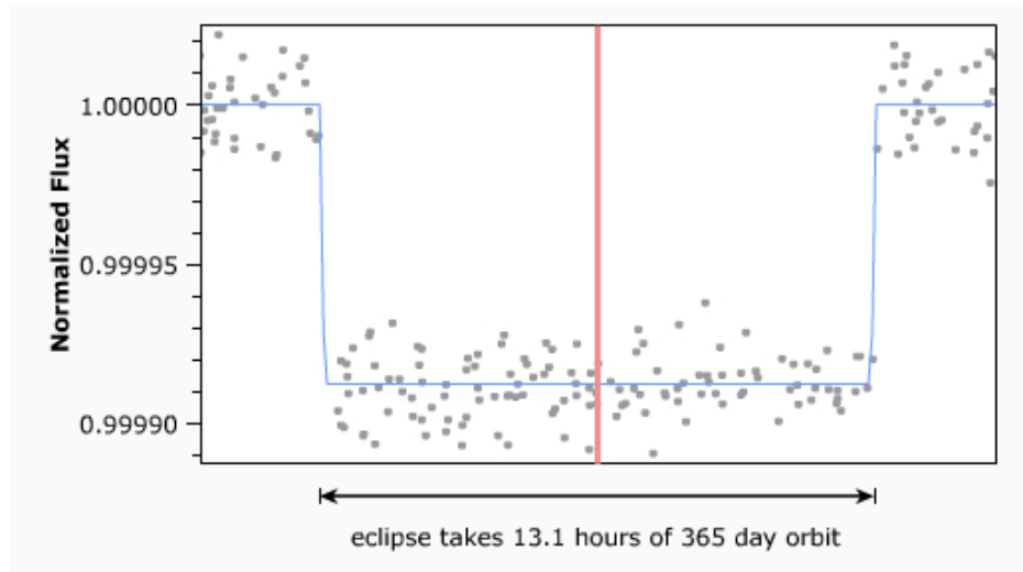
Figure 11.15: Transiting exoplanet #4.
