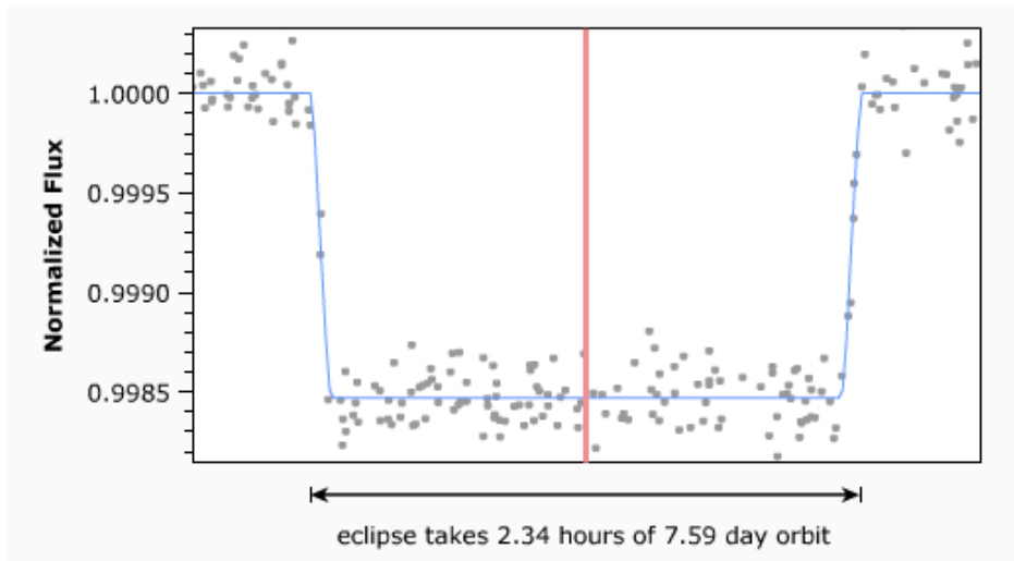
Figure 11.19: Transiting exoplanet #8.
