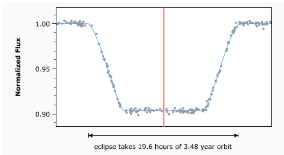
Figure 11.13: Transiting exoplanet #2.
