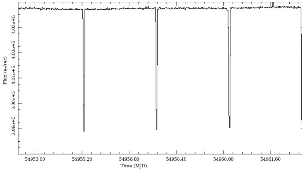
Figure 11.11: The light curve of Kepler 1b as measured by the Kepler satellite. The numbers on the y-axis are the total counts (how much light was measured), while the x-axis is “modified Julian days”. This is a system that simply makes it easy to figure out periods of astronomical events since it is a number that increases by 1 every day (instead of figuring out how many days there were between June 6 th and November 3 rd ). Thus, to get an orbital period you just subtract the MJD of one event from the MJD of the next event.
